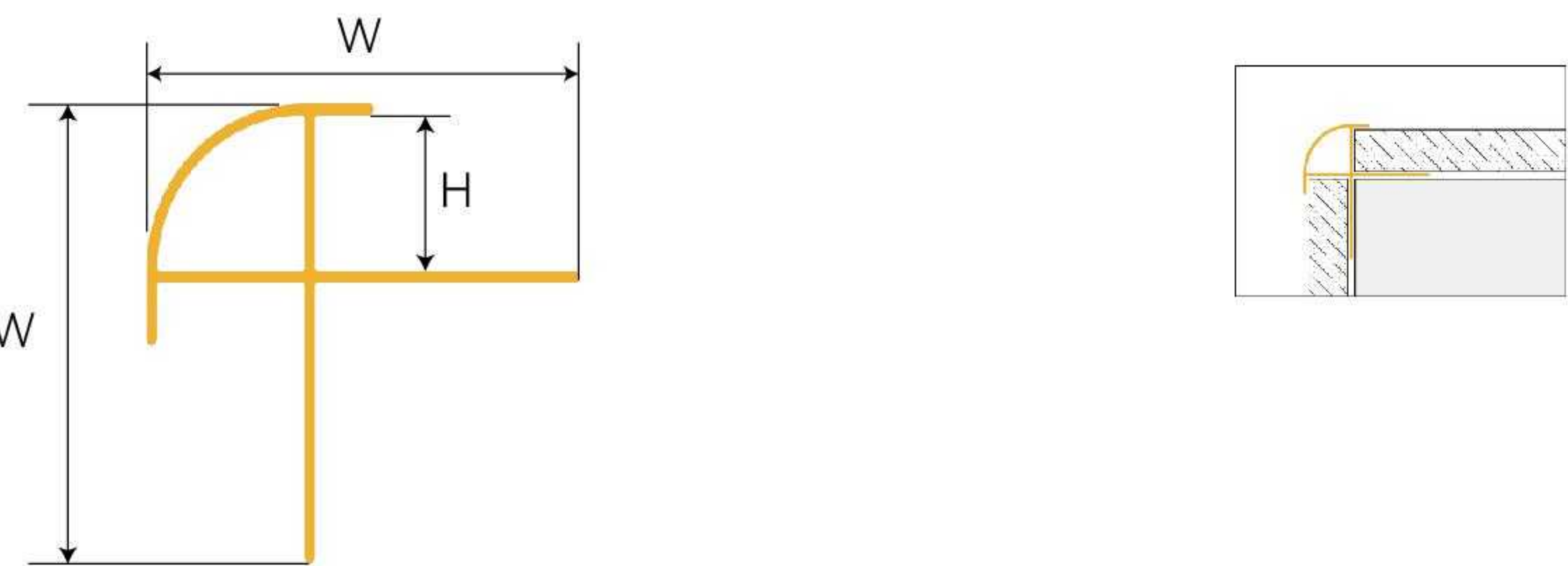
EXT-10.5-374 Wall Panel Trim
