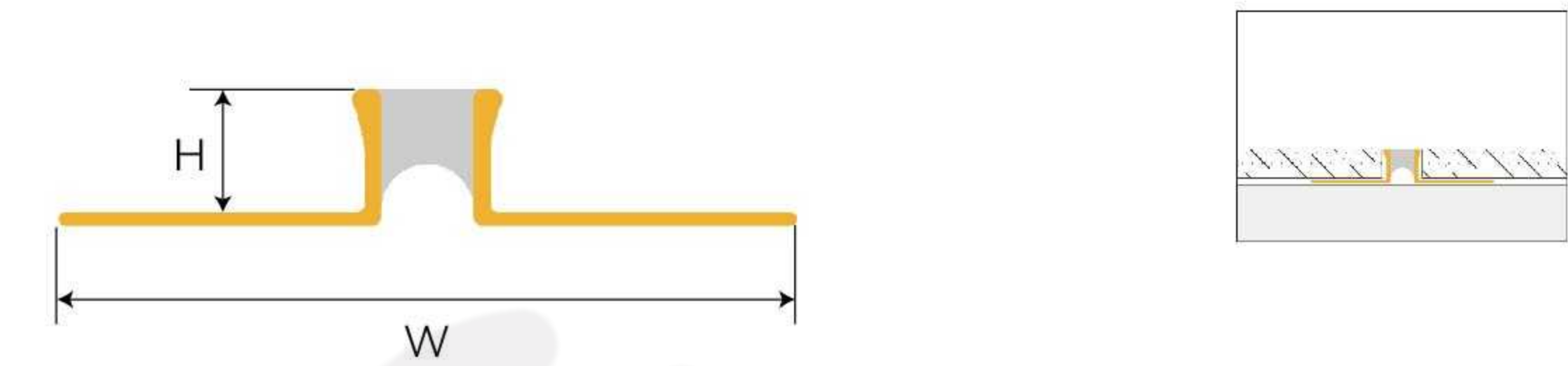
KK-08-160 Movement Joint
