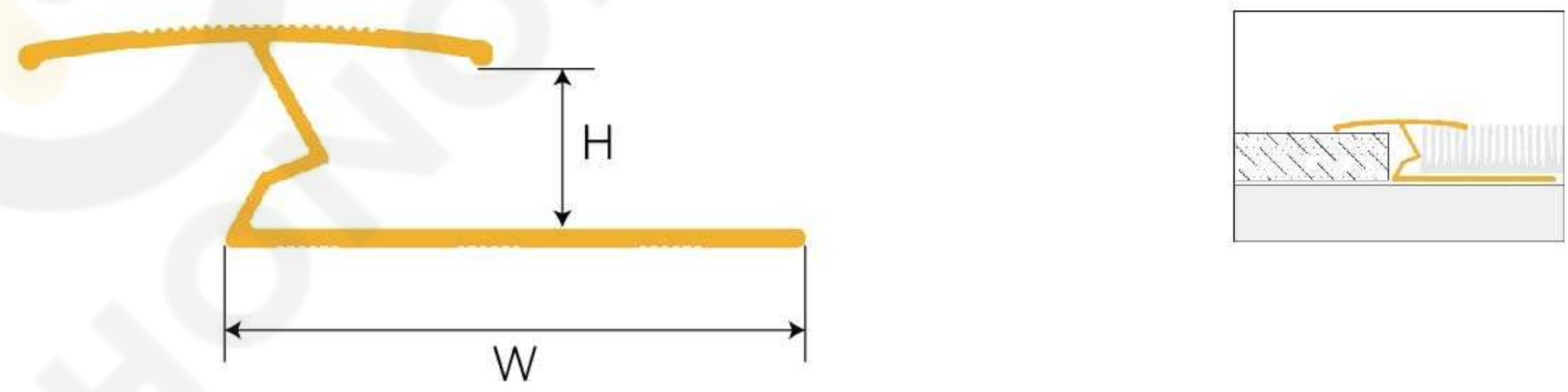
BD07-195-392 Carpet Trim
