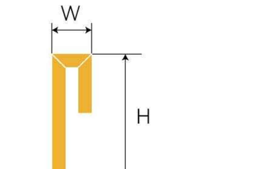
SS-005 Square Tile Trim
