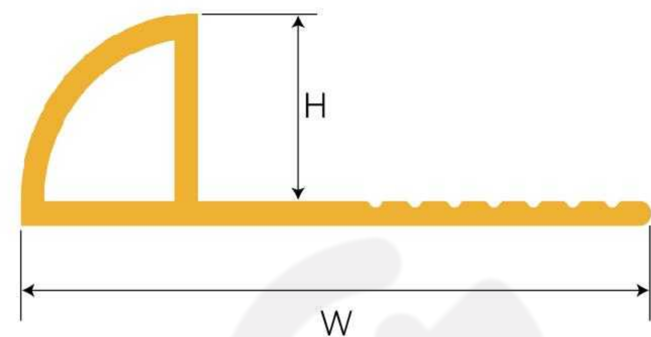
YF9-425-340 Round Tile Trim
