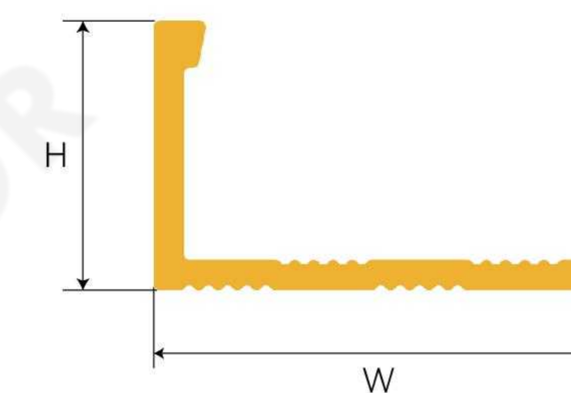
BRL-003 L Shape Tile Trim
