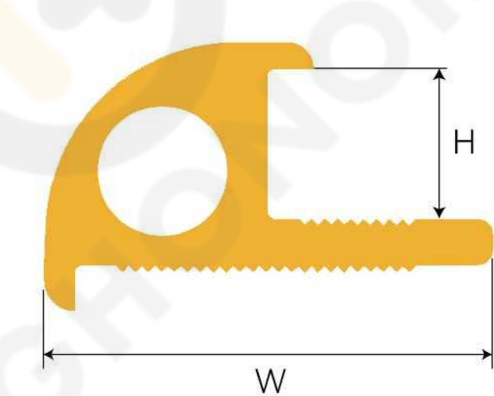
MP-001 Round Tile Trim
