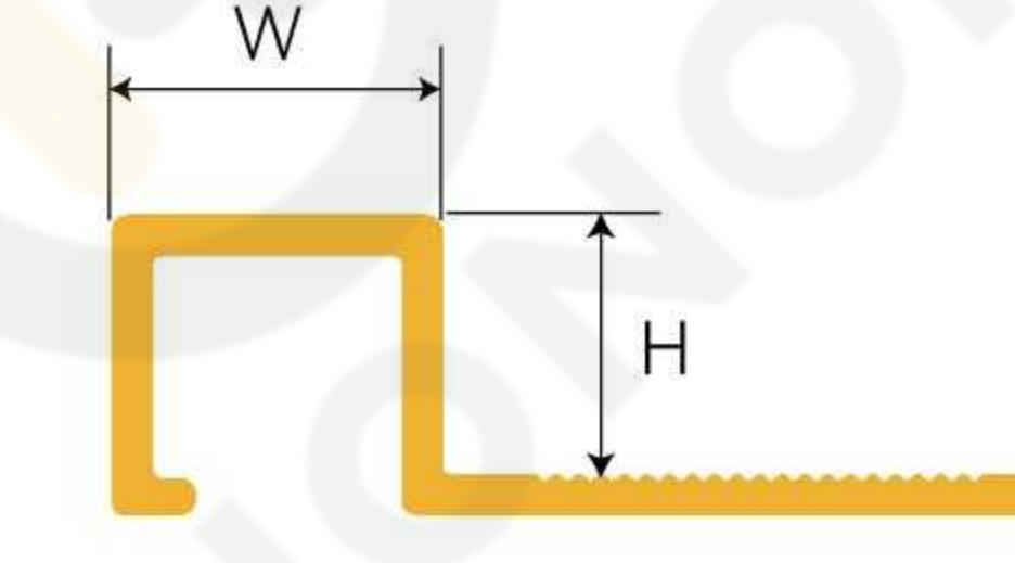
BRS-001 Square Tile Trim
