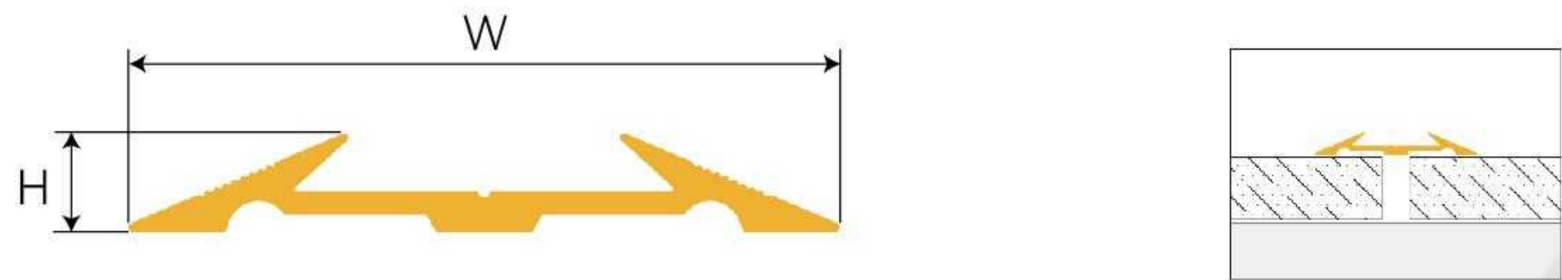
Y07-598-474 Floor Transition
