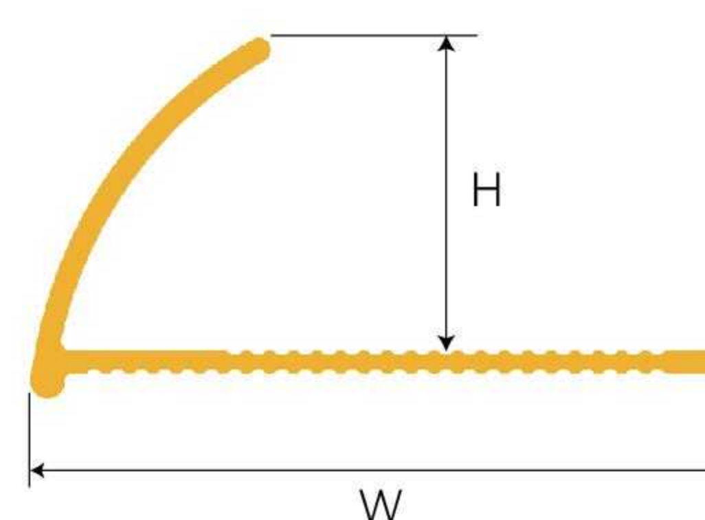
LS-C10-142 Round Tile Trim
