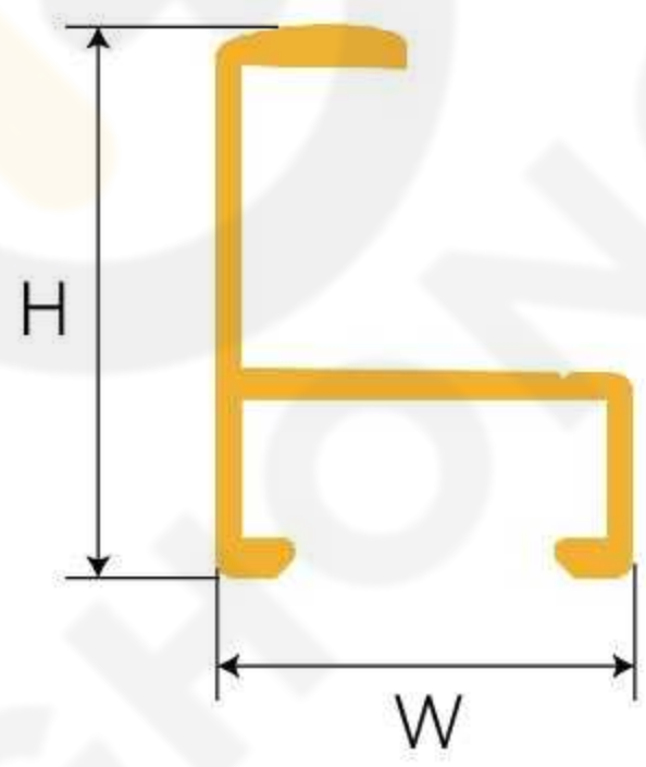
PF711-1-304 Photo/Picture/Mirror Frame
