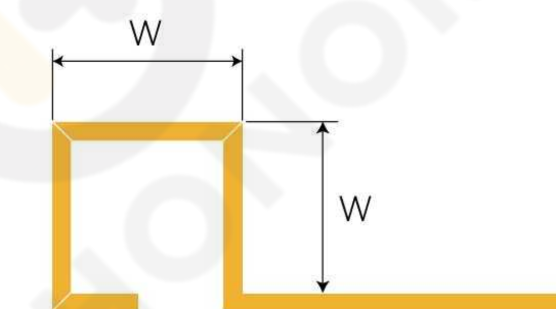
SS-004 Square Tile Trim
