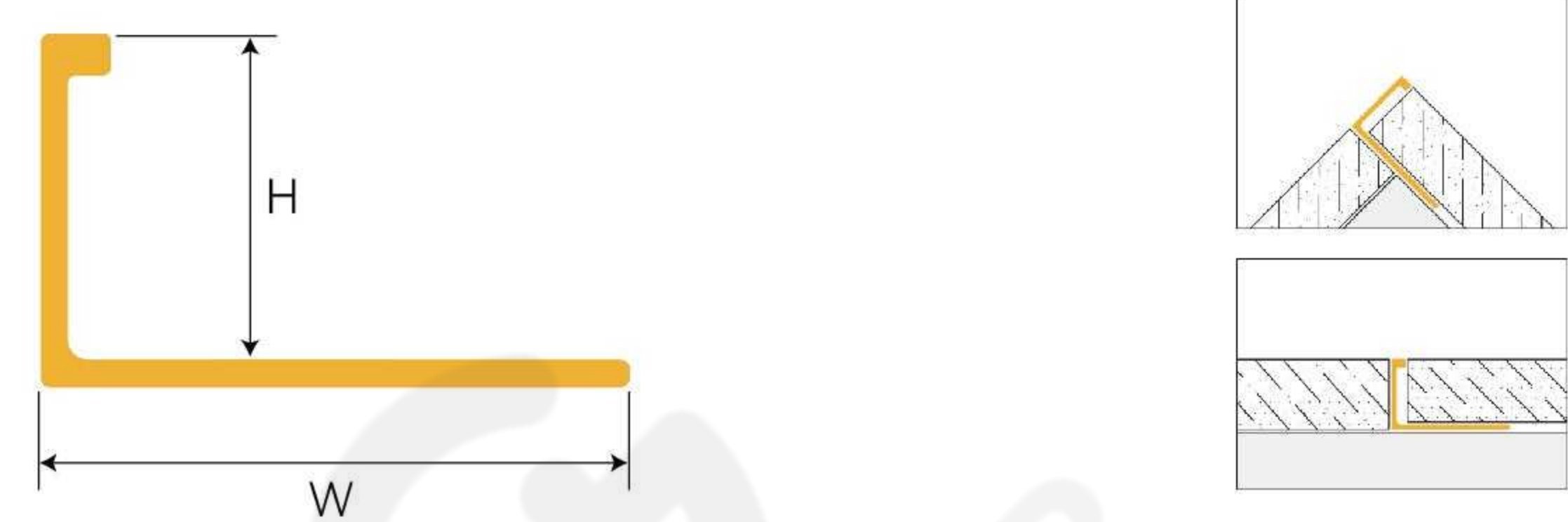
JKL10-245B-190 L Shape Tile Trim
