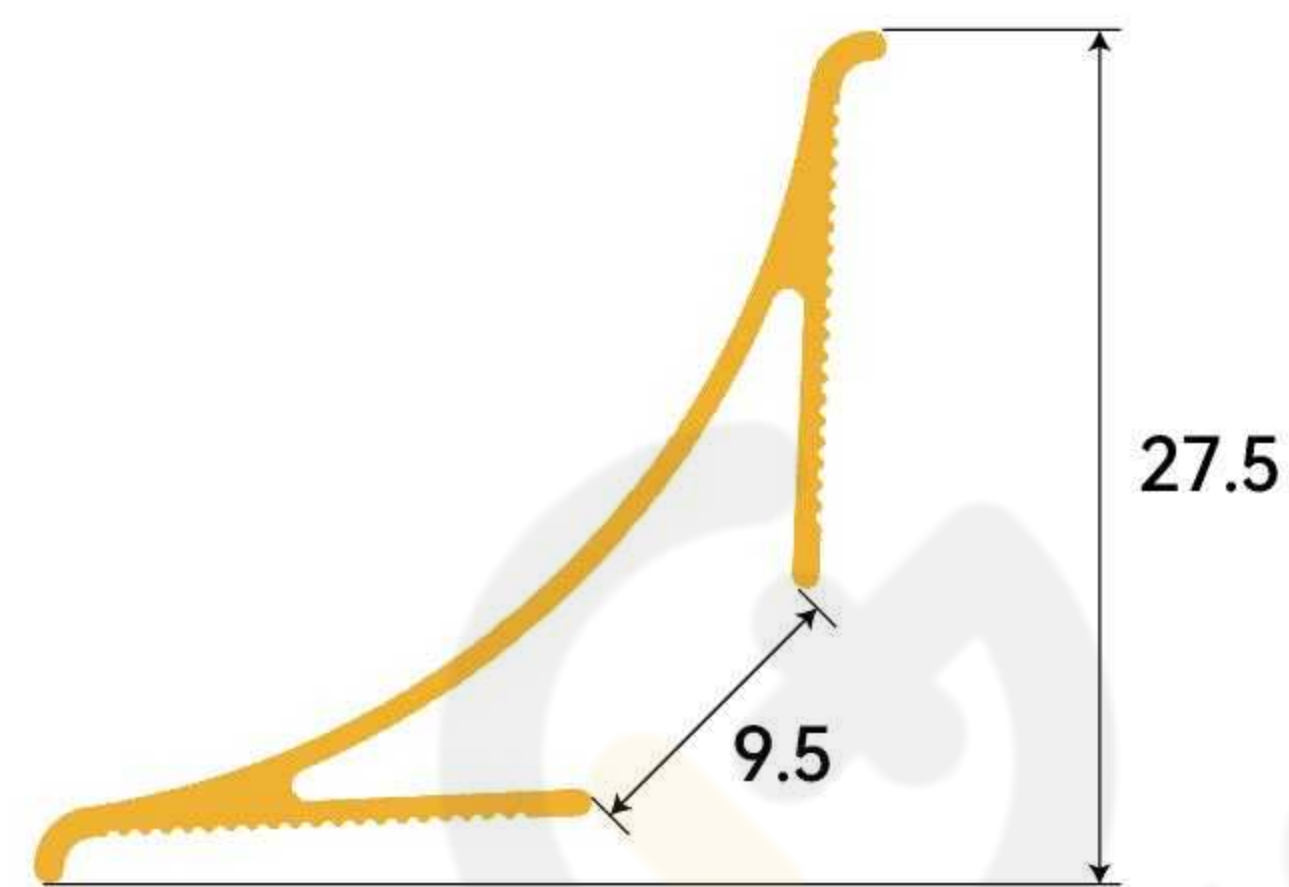
XBY-23-324 Internal Corner Trim
