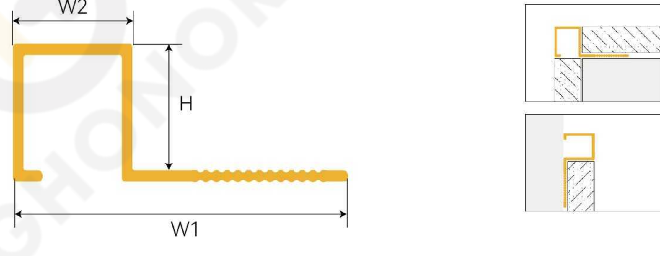
FK10x10-236 Square Tile Trim
