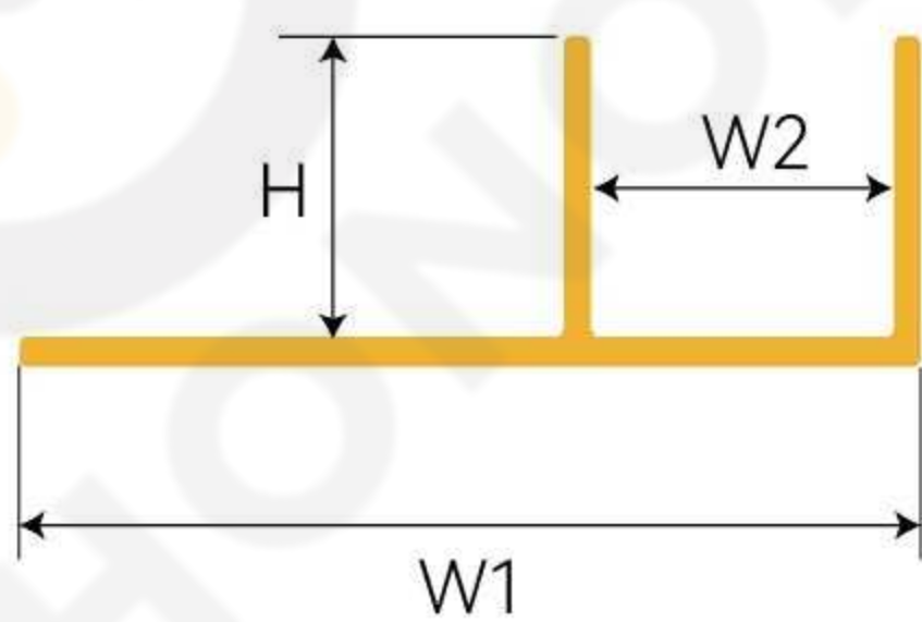
AK-F10-266 F-Shaped Profile
