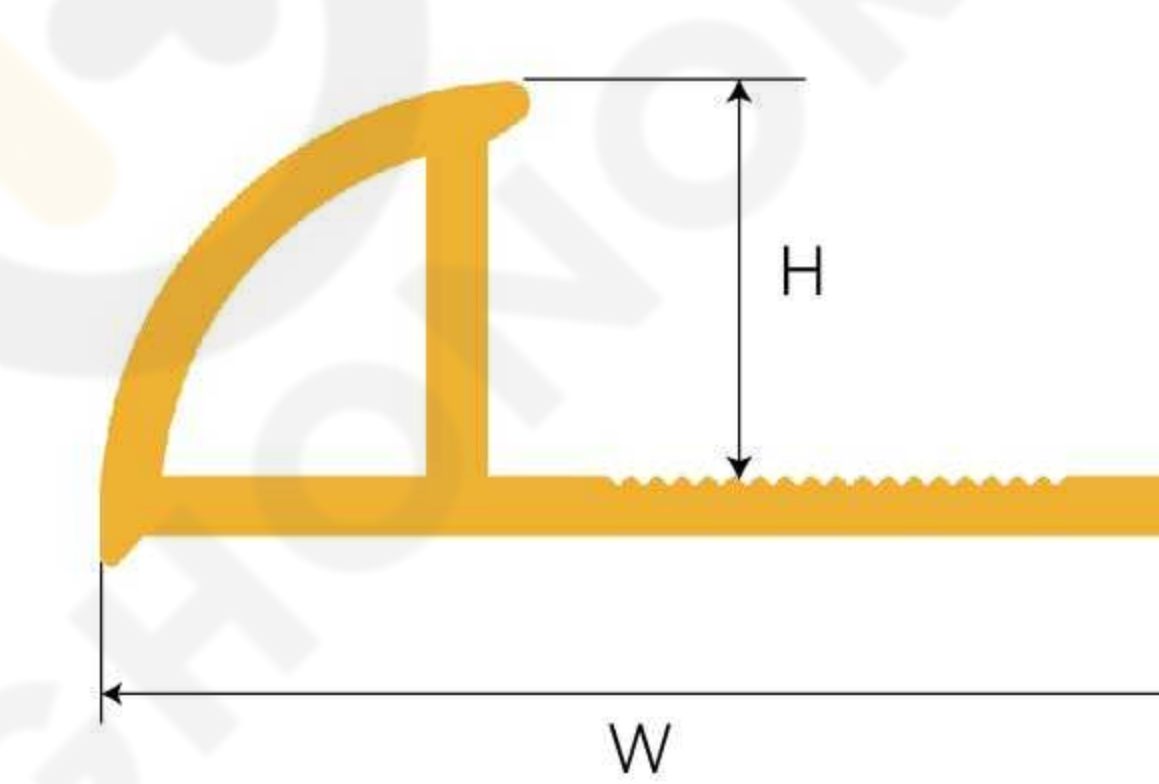
PVC-001 Round Tile Trim
