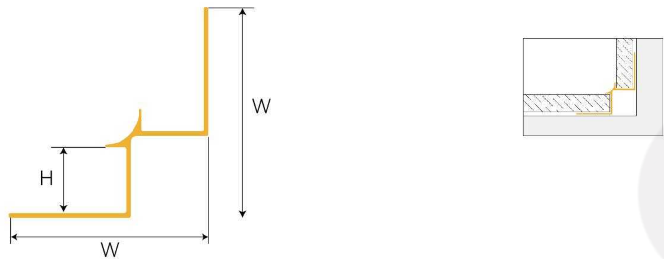
INT-10.5-314 Wall Panel Trim
