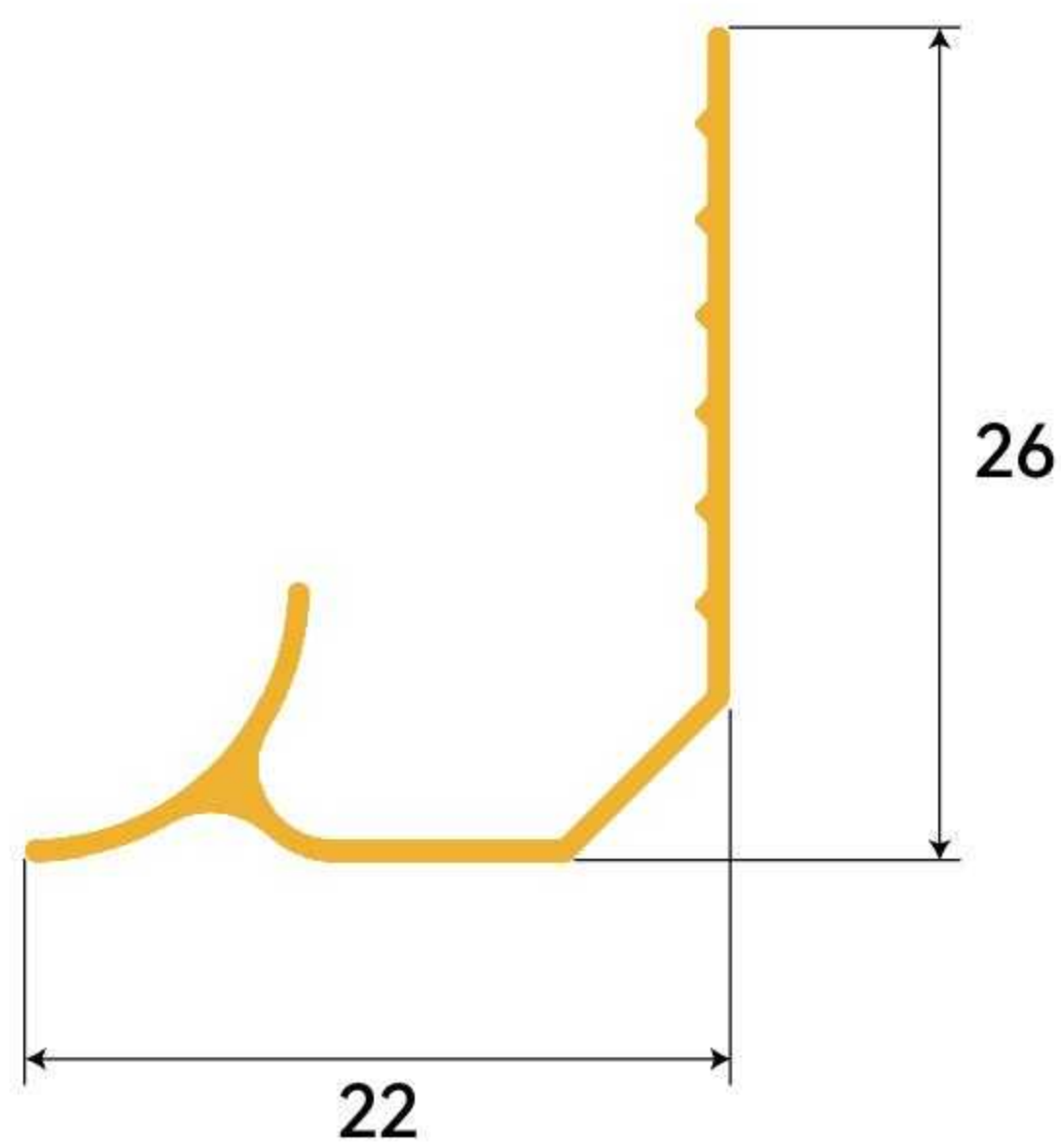
MH-Y22-214 Internal Corner Trim
