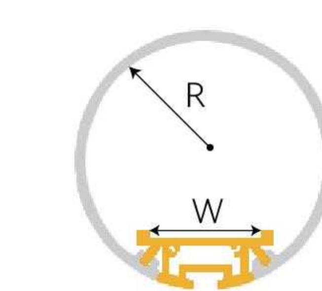
Φ60 LED Profile
