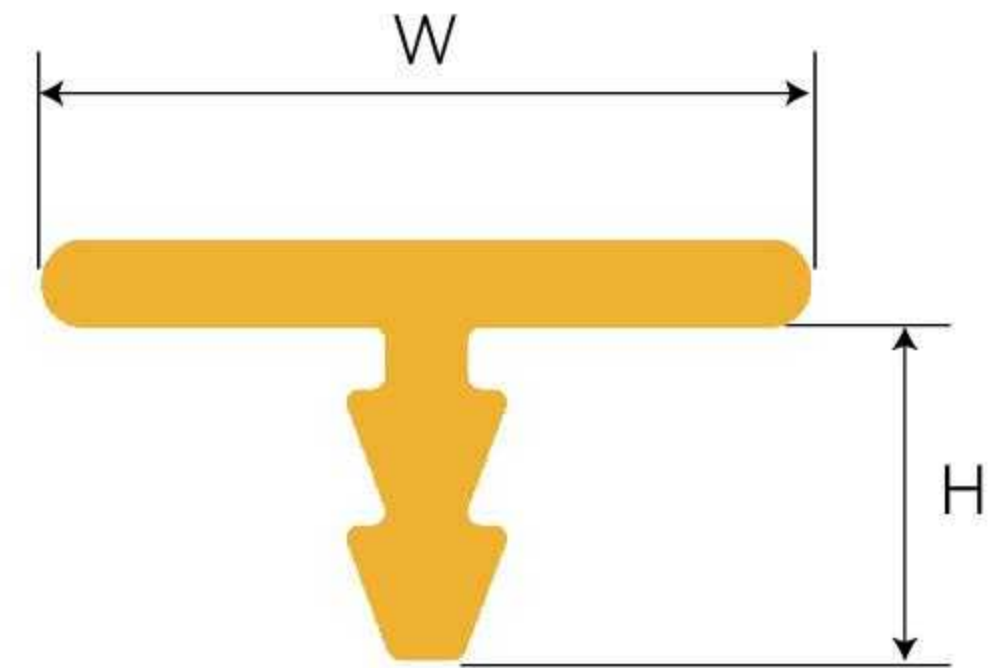
ADI-T12-130 T Shape Tile Trim
