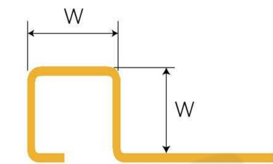
SS-001 Square Tile Trim
