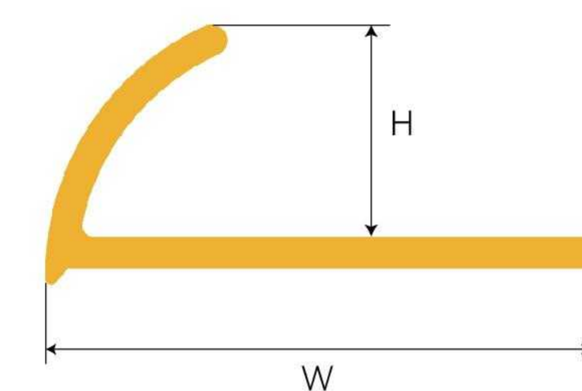
PVC-002 Round Tile Trim
