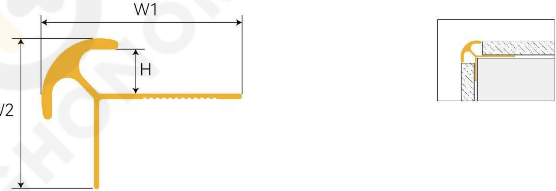
N859-168 Wall Panel Trim
