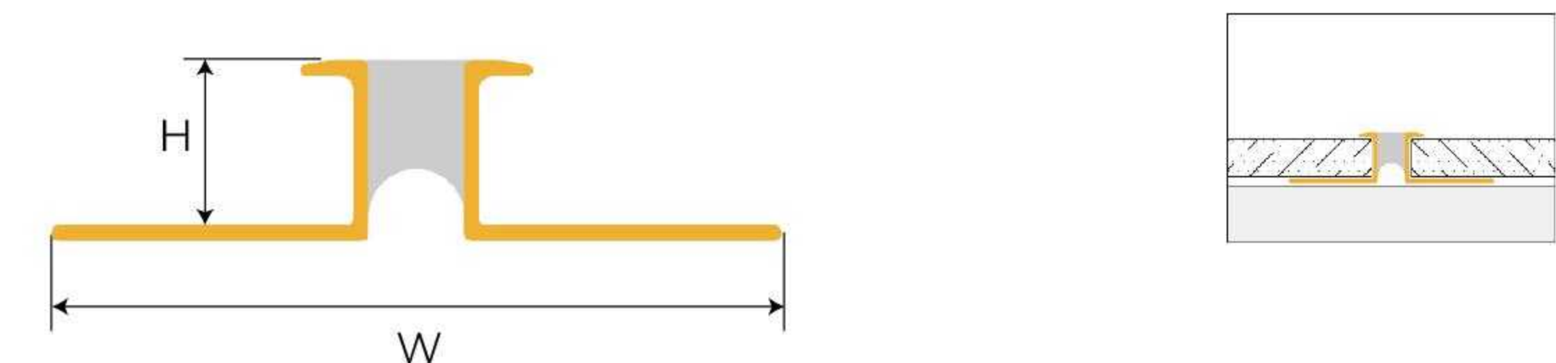
ALM-008-244 Movement Joint
