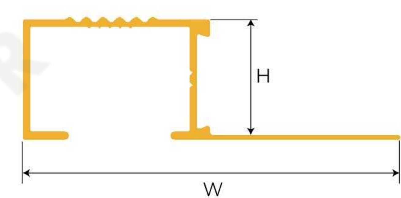
FH13-410A-328 Stair Nosing
