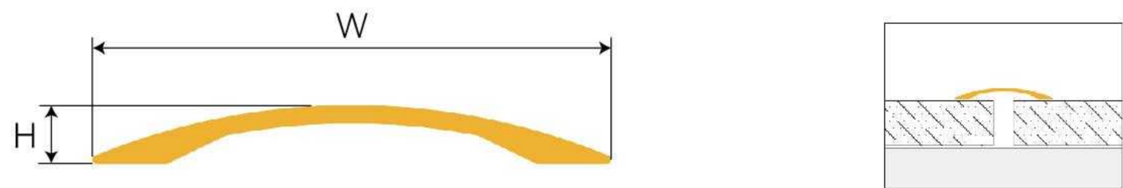
KSF35-260 Floor Transition
