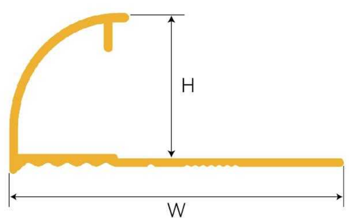
HS-YC10-160 Round Tile Trim
