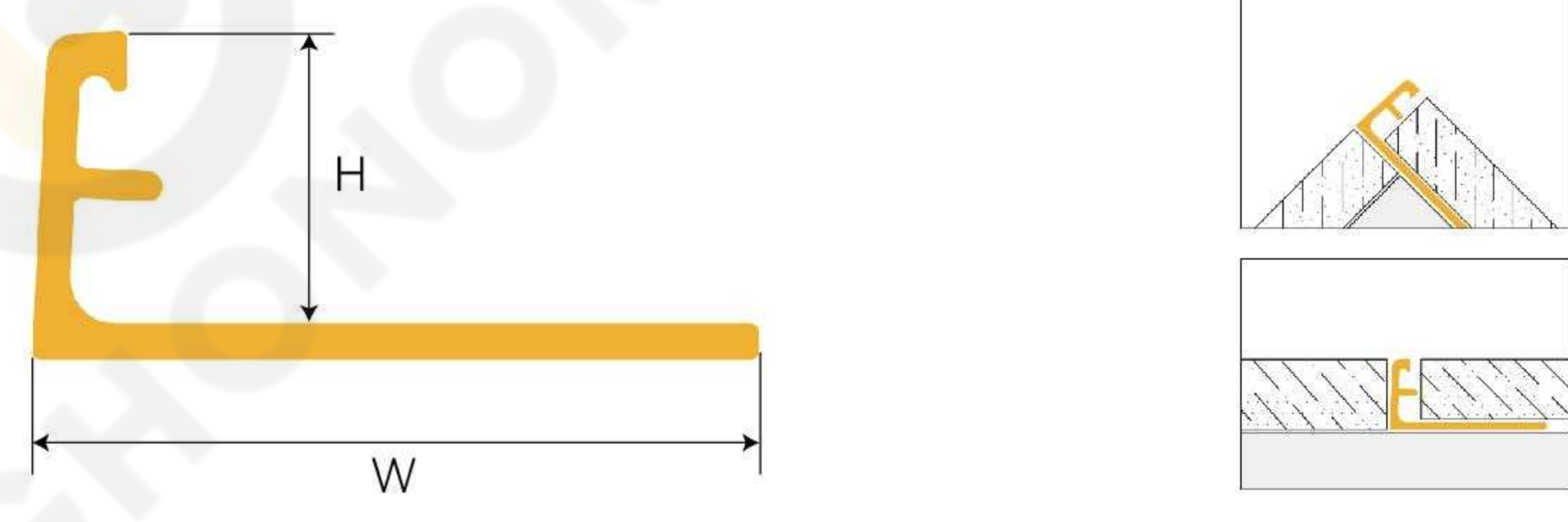
WA-L95N-256 L Shape Tile Trim
