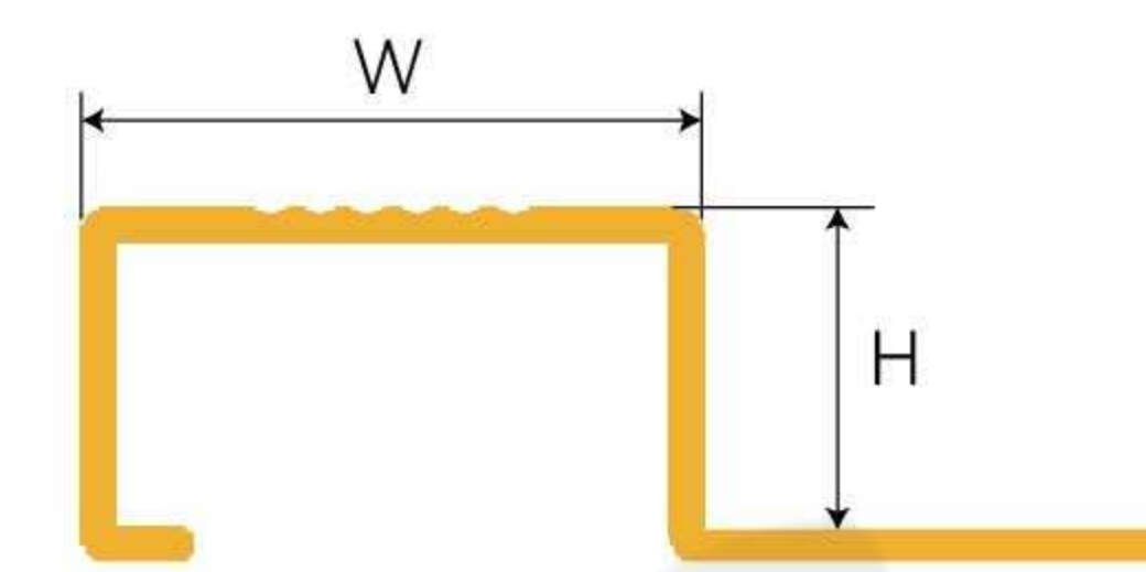
SJ-013 Stair Nosing
