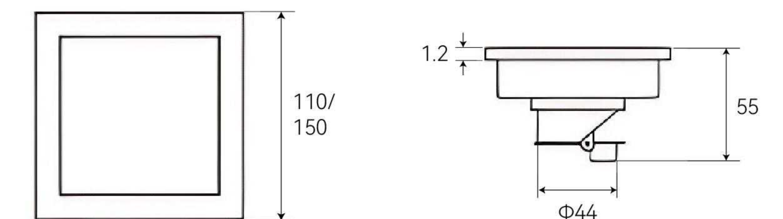
FD-005 Stainless Steel
