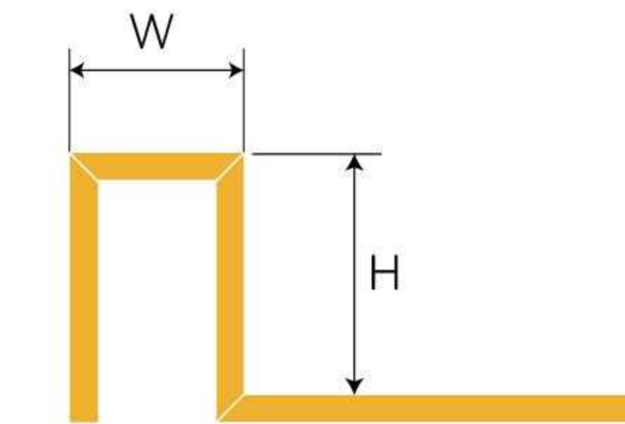
SS-003 Square Tile Trim
