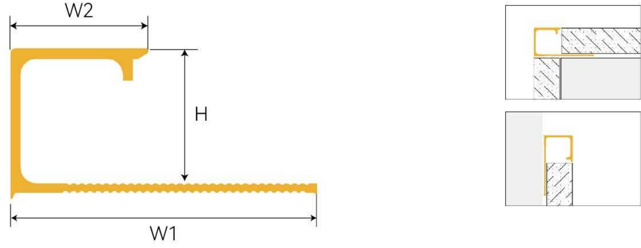
AS043-350-280 Square Tile Trim
