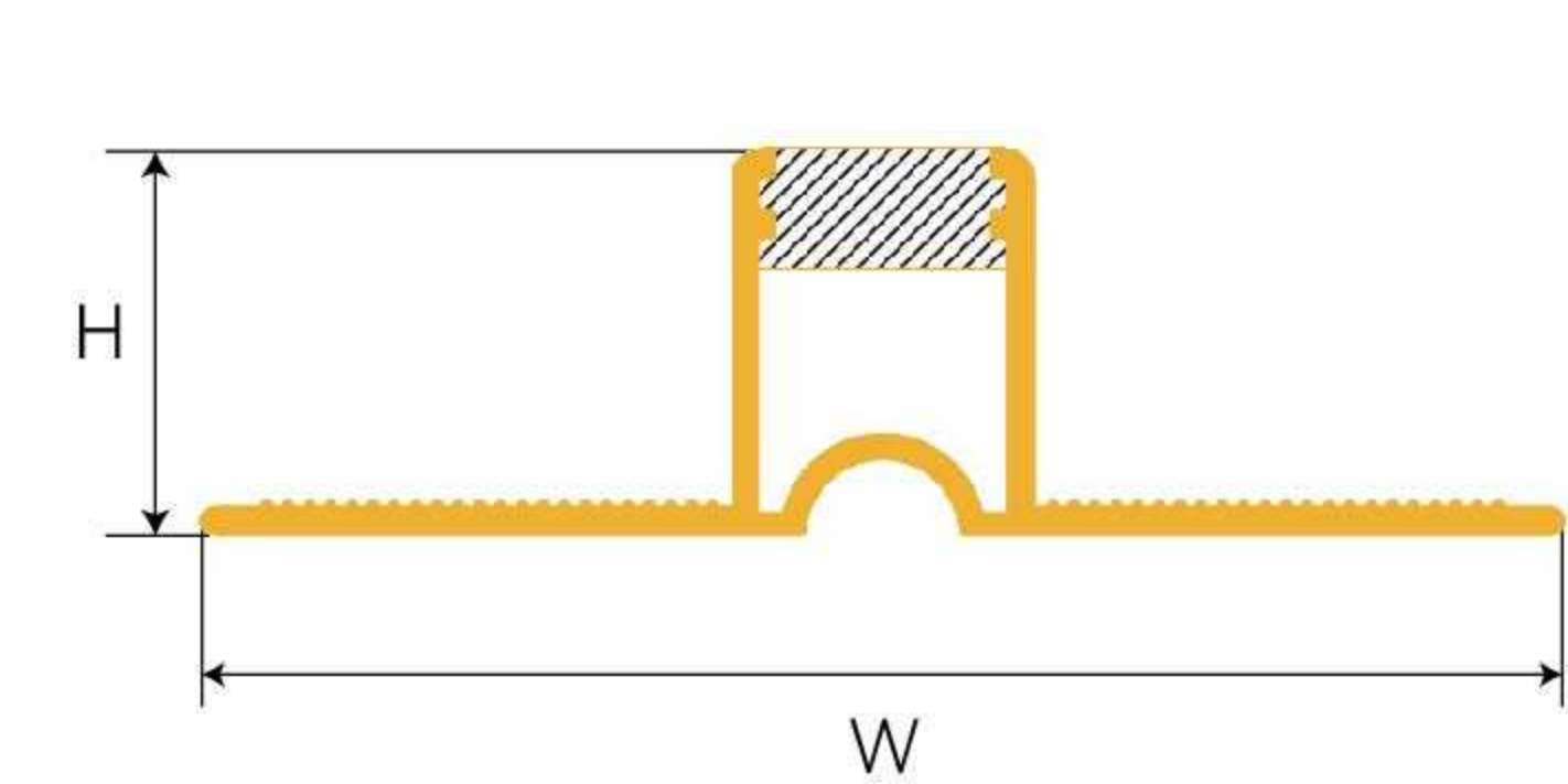
PVC-005 Movement Joint
