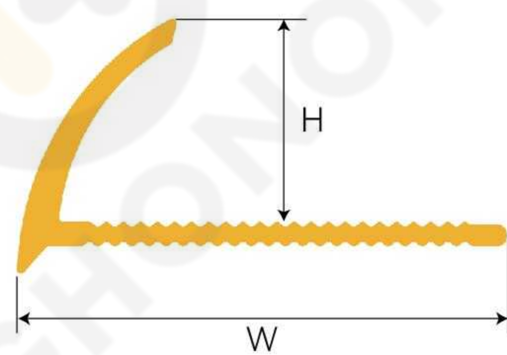
BK9-240-192 Round Tile Trim
