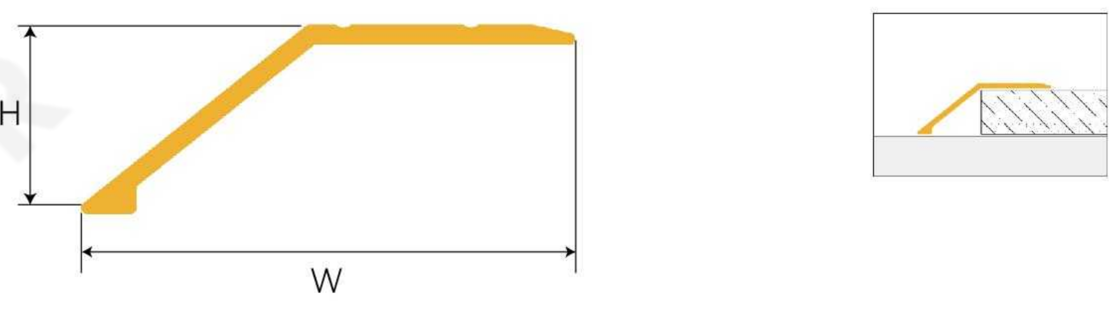
HW06-550-440 Floor Transition
