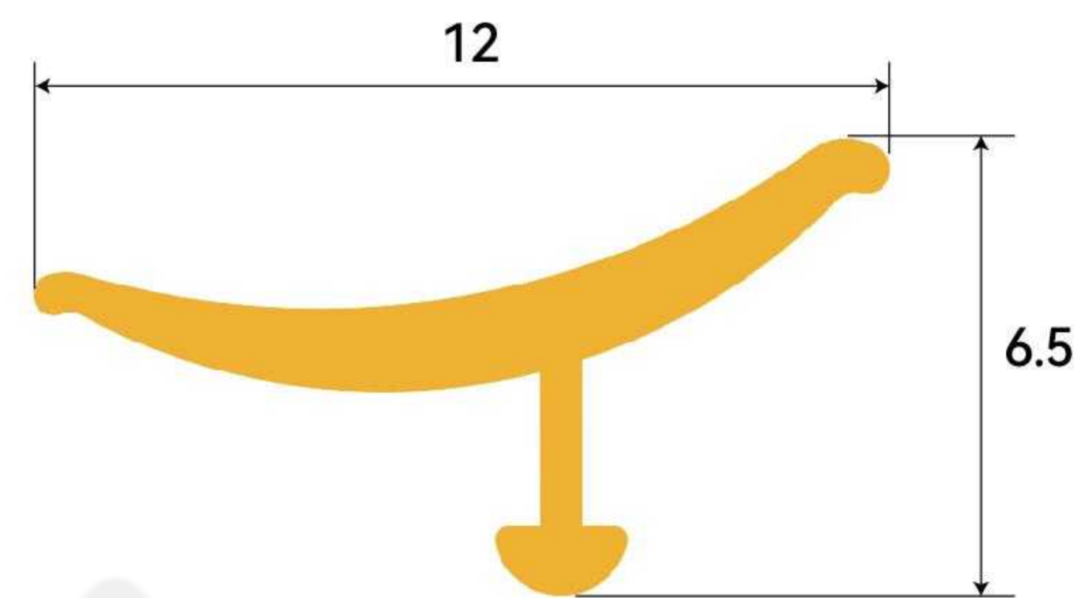
YA12-88 Internal Corner Trim
