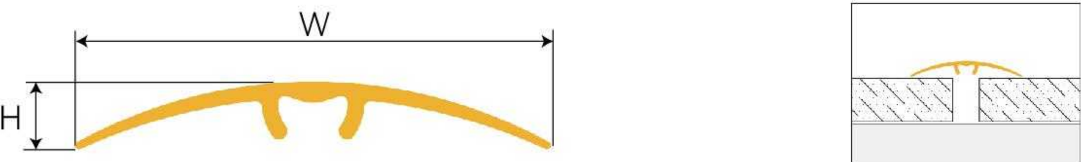
BC317-254 Floor Transition
