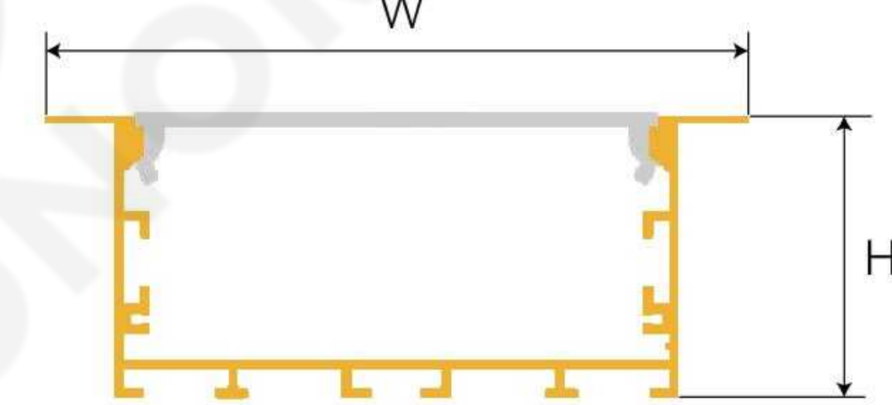
7035A LED Profile
