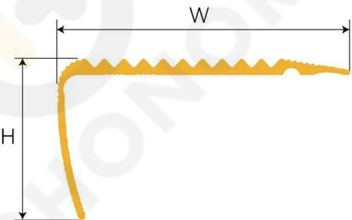
X006-472 Stair Nosing
