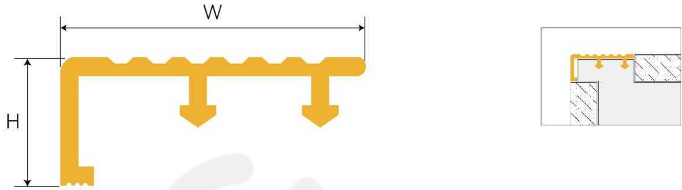
E50-1655-1324 Stair Nosing
